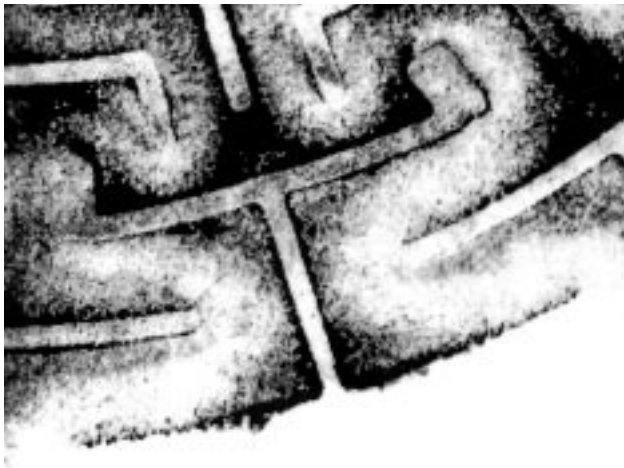
Actual gaseous flow through Raven trim as recorded in DeZURIK/Copes-Vulcan's Technical Center.
