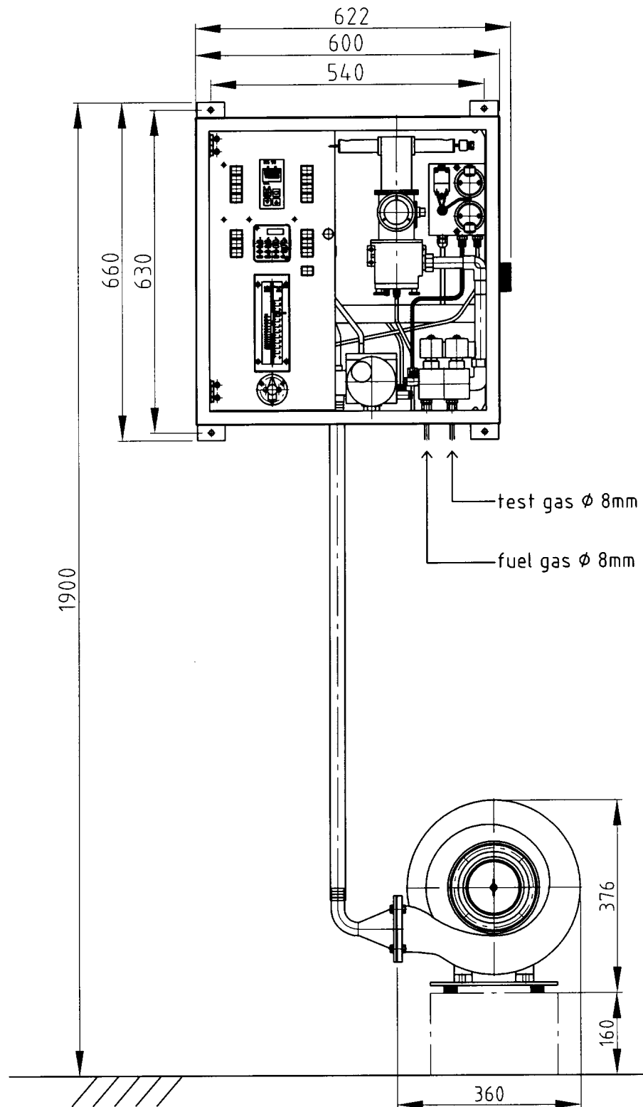
Gas Analyser WI for Wobbe-Index or net calorific value
