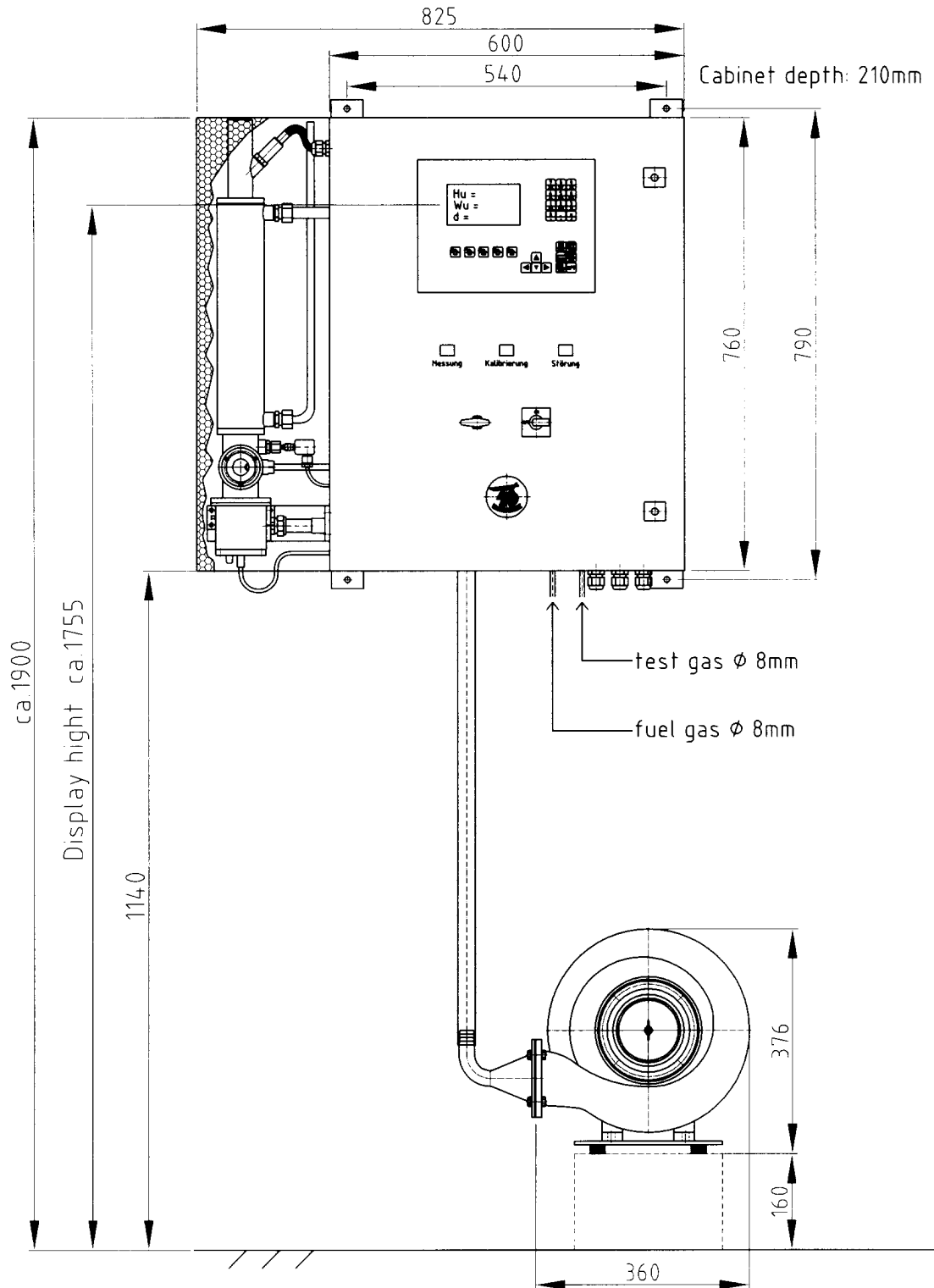
Gas Analyser RBM 2000 with air fan
